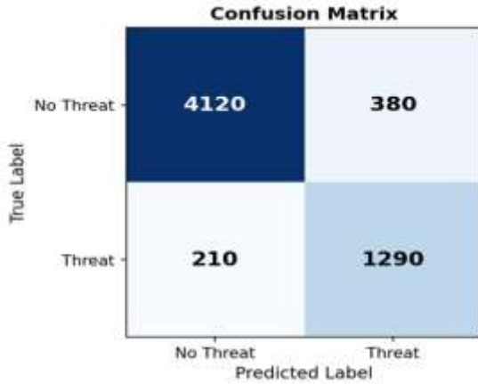
Fig.3. Confusion Matrix of Threat Detection Module
